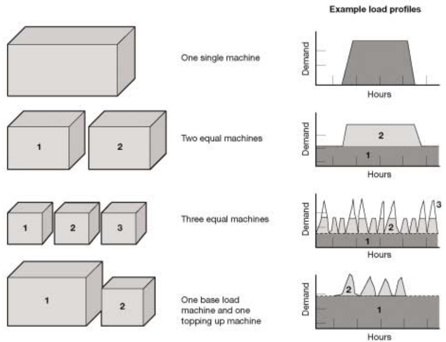
Figure 1. Meeting Demand Patterns Efficiently with Combinations of Compressors
